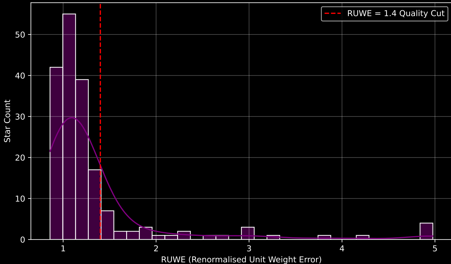
GAPOGEE DR17 Field [138+64_MGA] RUWE Distribution (n= 183)
