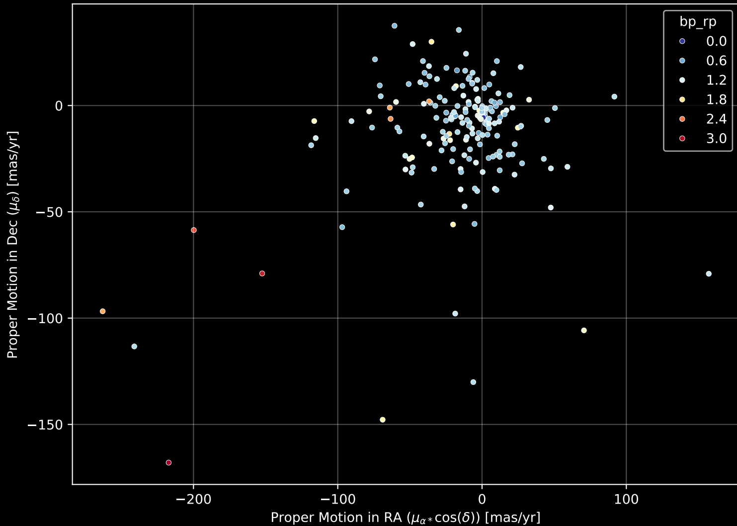
APOGEE DR17 Field: [138+64_MGA] Proper Motion Diagram (n= 192)
