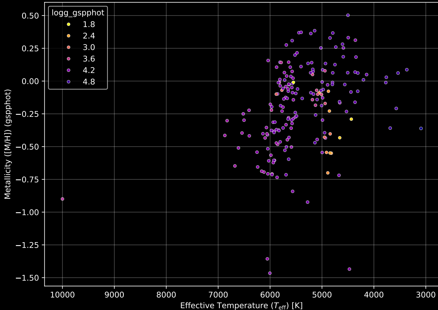
APOGEE DR17 Field: [138+64_MGA] Stellar Population Parameters (n= 192)
