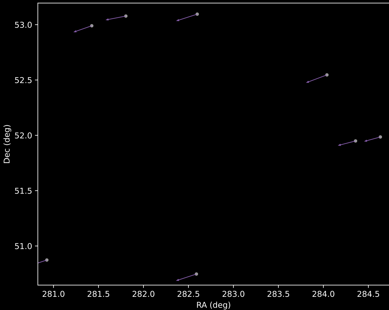
APOGEE DR17 Cluster 8 Proper Motion Vectors (n=8)
