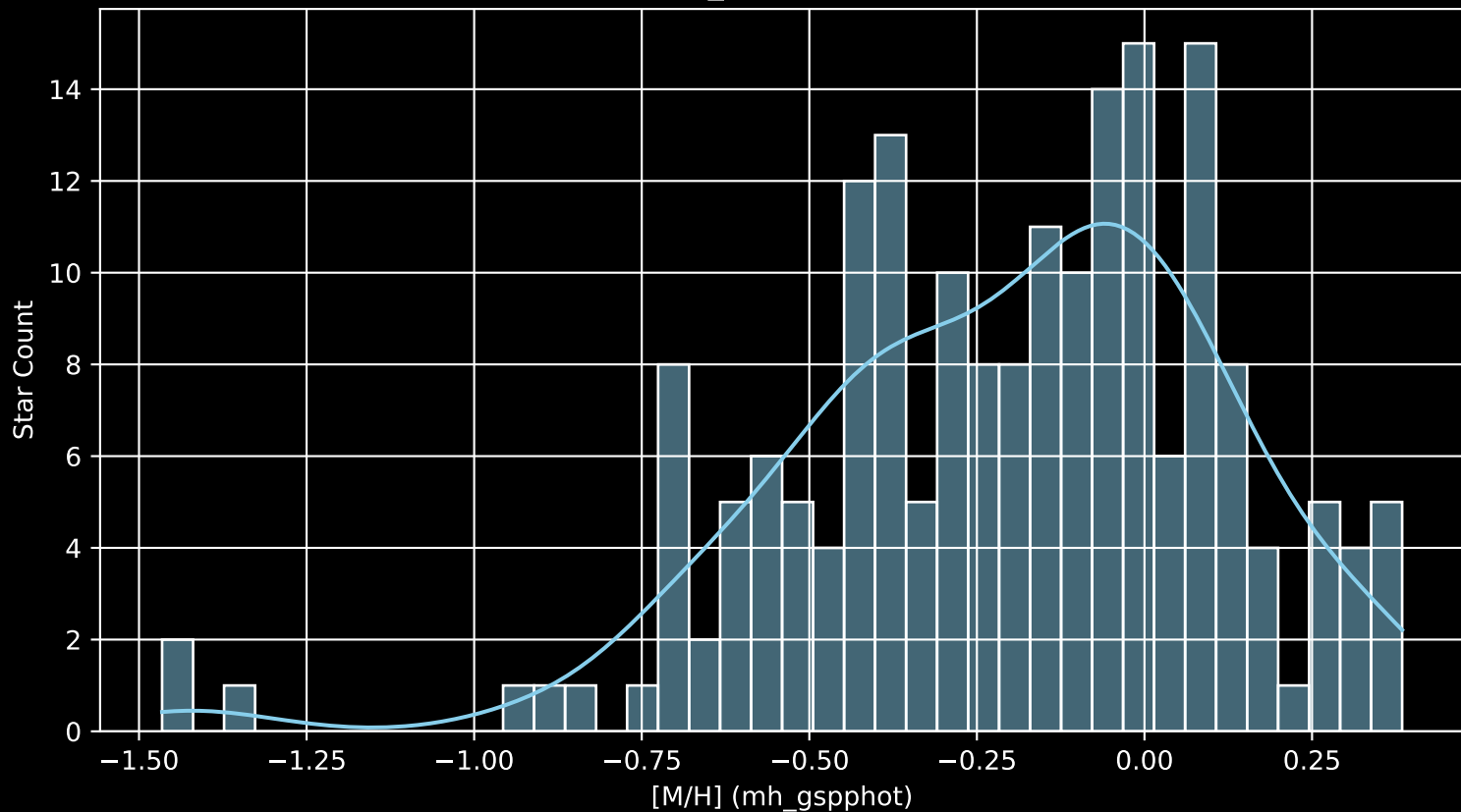
APOGEE DR17 Field: [138+64_MGA [M/H] (mh_gspphot) (n= 191)
