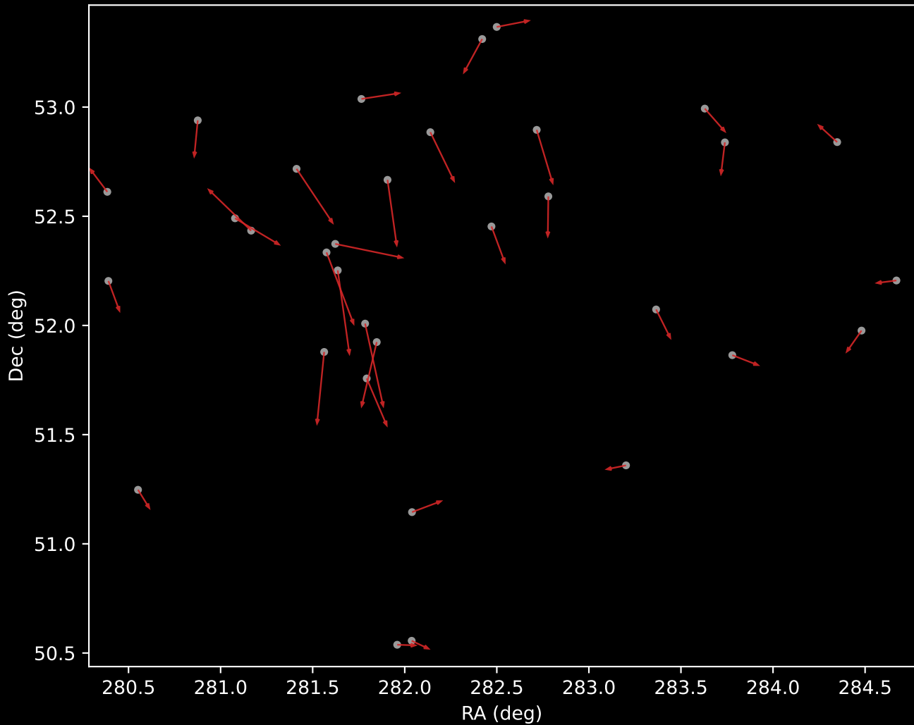
APOGEE DR17 Cluster 6 Proper Motion Vectors (n=33)
