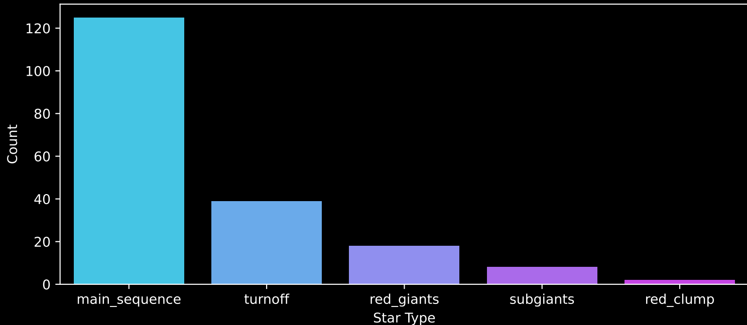
APOGEE DR17 Field: [138+64_MGA] Count plot of Star Type
