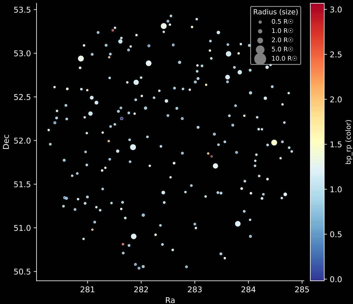
APOGEE DR17 Field: [138+64_MGA] Stars: 192
