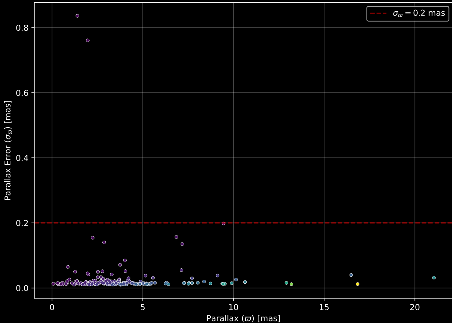
APOGEE DR17 Field: [138+64_MGA] Parallax Quality (n= 192)
